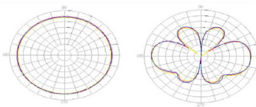
H Plane - Azimuth
