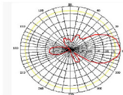
E Plane - Vertical
