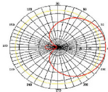
H Plane - Azimuth
